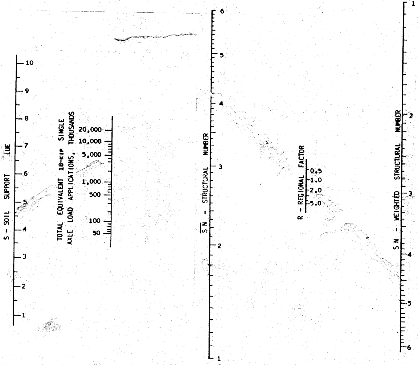
Design Chart for Flexible Pavements, p_t = 2.5
